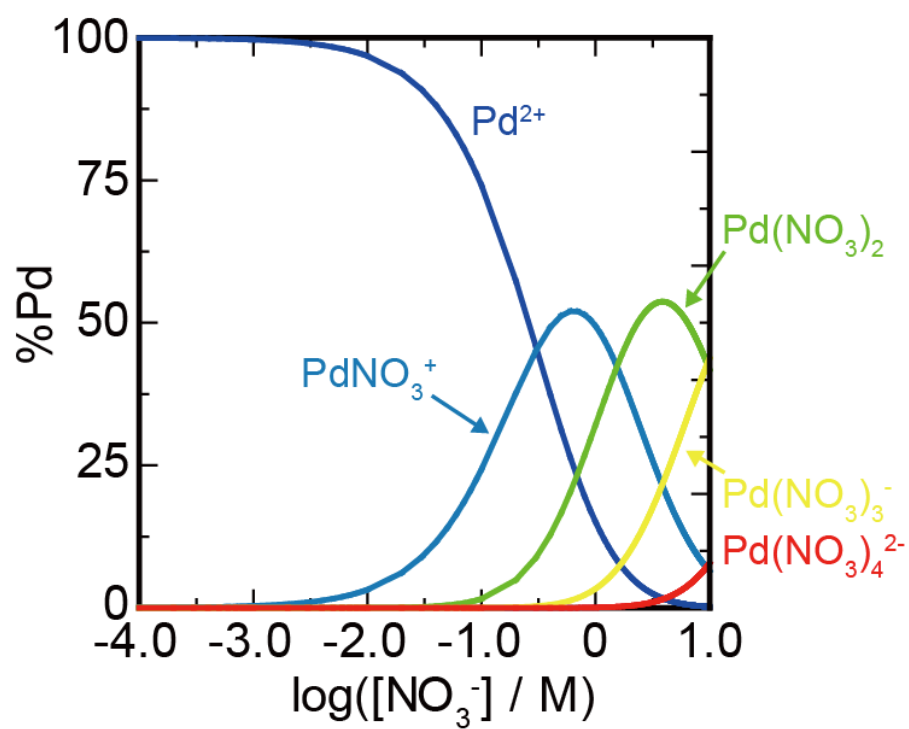
S3 Palladium species ratio at different nitrate concentrations. [27]
