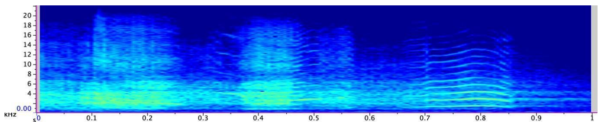
Sulphur-crested Cockatoo Croak Spectrogram.
