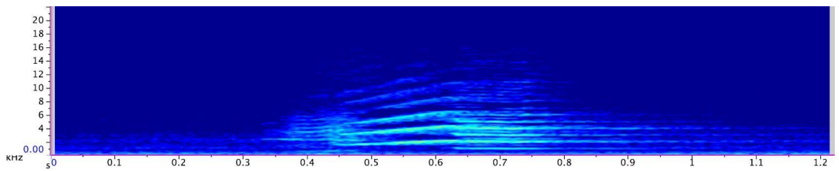
Sulphur-crested Cockatoo Rain Call Spectrogram.
