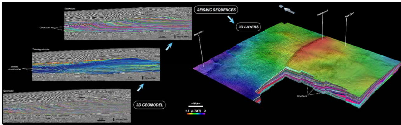
Figure 3: High-resolution sequence stratigraphic interpretation workflow using PaleoScan ® . From the 3D geomodel and the thinning attribute, seismic sequences are identified from which 3D layers can be generated. Data courtesy of TGS.
