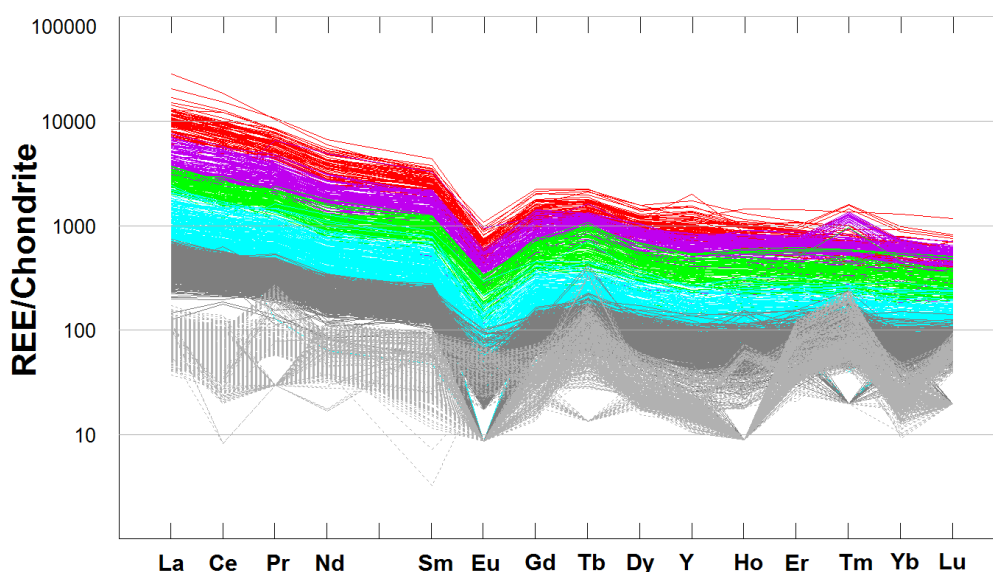
Figure 2. Chondrite-normalised graph of alkaline intrusive-hosted REE deposit. (Colours highlight various TREO% ranges: >1%, 1-0.5%, 0.5-0.3%, 0.3-0.1%, 0.1 – 0.05% & <0.05% )
