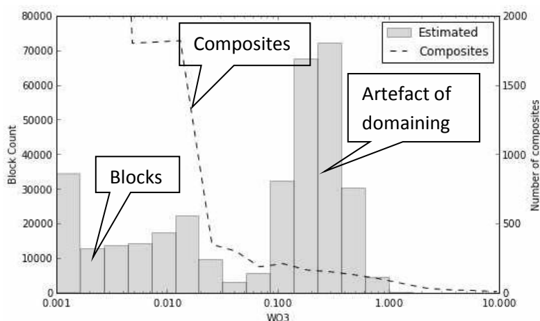
Figure 3. Conflict between populations of blocks and composites due to over-domaining (Left hand Y-axis is the block count and the right hand Y-axis is the number of underlying composites upon which the estimate is based. The X-axis shows the grade of the variable being estimated (in this case WO_3 ). Kindly contributed by Mr R Osborn, H&S Consultants).
