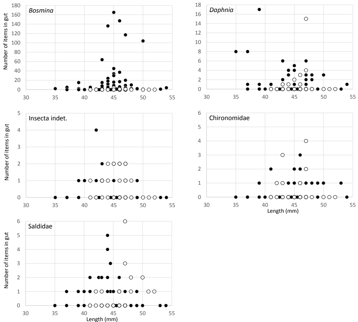
Fig. S1. Relationships between length of juvenile Galaxias maculatus and the number of items in the guts for dominant invertebrate taxa and at Mercer (closed circles) and Tuakau (open circles), lower Waikato River.
