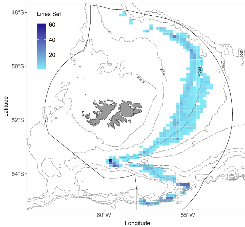
Fig. S1. Spatial distribution of longline fishing effort (number of lines set per 0.1 \times 0.1^\circ grid square; n = 2236 ) during the study period (June 2016–October 2021) in the Falkland Islands Conservation Zones.
