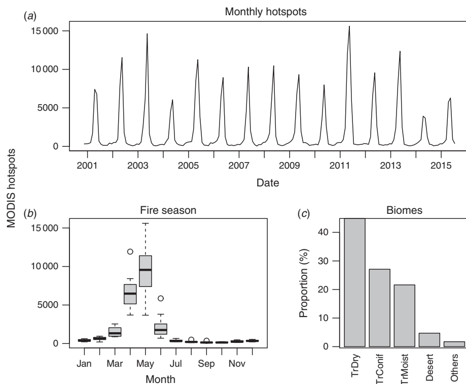
Fig. 1. Recent fire activity in Mexico (2001–2015) estimated from the monthly number of active fires recorded by the Terra satellite (MODIS hotspots). (a) Temporal variability (x-axis ticks indicate the beginning of the year). (b) Fire seasonality; the flammable season is concentrated into four months (March–June), with a peak in April–May (the end of the dry season). (c) Proportion of active fires in each biome (TrDry: tropical dry broadleaf forests; TrConif: tropical coniferous forests; TrMoist: tropical moist broadleaf forests; Desert: deserts and xeric shrublands; Others). The MODIS fire data was downloaded from the University of Maryland (MCD14ML, http://modis-fire.umd.edu , accessed 10 November 2015), intersected with a country map and the biome map produced by the World Wildlife Fund (Pausas and Ribeiro 2013), and aggregated at the monthly scale.
