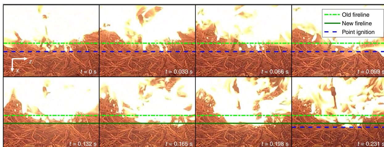
Fig. 7. Point ignitions and corresponding fireline movement in Pinus palustris at U = 0.42 \text{ m s}^{-1} seen from back view.
