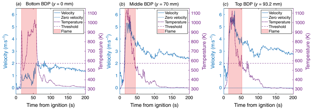
Fig. 11. Comparison of velocity and temperature measured by BDP at various vertical locations, (a) y = 0 mm, (b) y = 70 mm and (c) y = 93.2 mm, for U = 1.38 \text{ m s}^{-1} for Pinus palustris .
