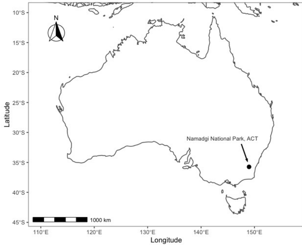
Figure S1. Observations were made in Namadgi National Park in the Australian Capital Territory (ACT) situated in the south-eastern region of Australia.
