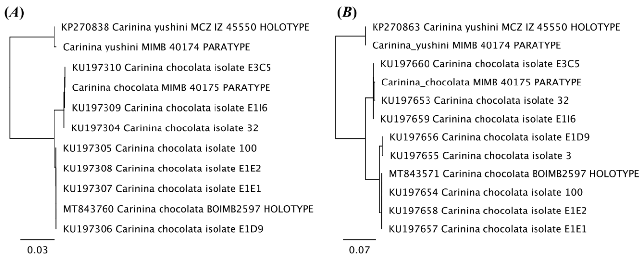
Fig. S1. Distance (NJ) trees including sequences of Carinina yushini , sp. nov. and Carinina chocolata , sp. nov. A. 16S rRNA. B. Cytochrome Oxidase I. Scale bars show uncorrected sequence divergence ( p -distances).
