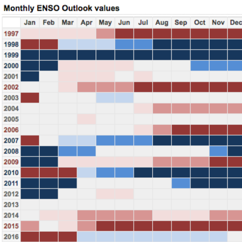
Fig. S1. Monthly likelihood of El Niño (red) and La Niña (blue) events on the basis of El Niño–Southern Oscillation (ENSO). The degree of likelihood increases from light to medium to dark colours, with dark colours representing a confirmed El Niño or La Niña event. Red- or blue-coloured years indicate that the year was dominantly an El Niño or La Niña year respectively. The figure has been adapted from http://www.bom.gov.au/climate/enso/outlook/#tabs=ENSO-Outlook-history (accessed 1 October 2017).
