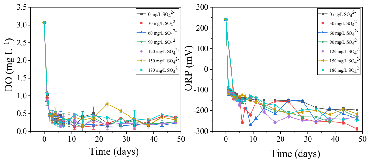
Fig. S1. Dynamic change of DO and ORP in the water column during the incubation.
