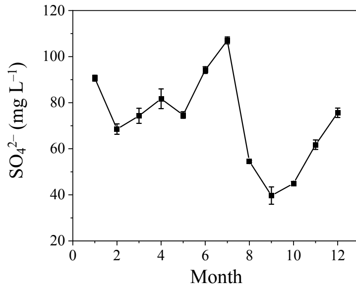
Fig. S4. Annual variation of SO 4 2- concentration in overlying water of Taihu Lake.
