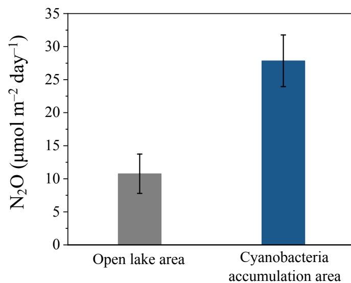
Fig. S3. N 2 O release fluxes across water-air interface of cyanobacteria accumulation area and open lake area in Lake Taihu collected by floating static chambers.
