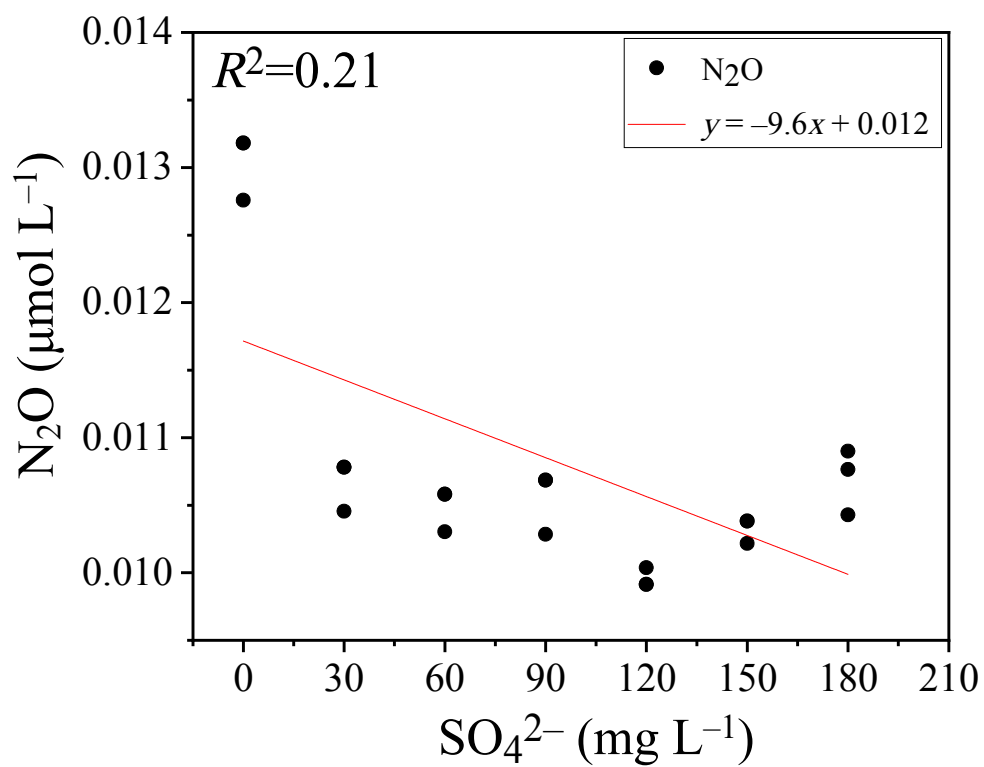
Fig. S2. The correlation between initial \text{SO}_4^{2-} concentration and maximum \text{N}_2\text{O} concentration.
