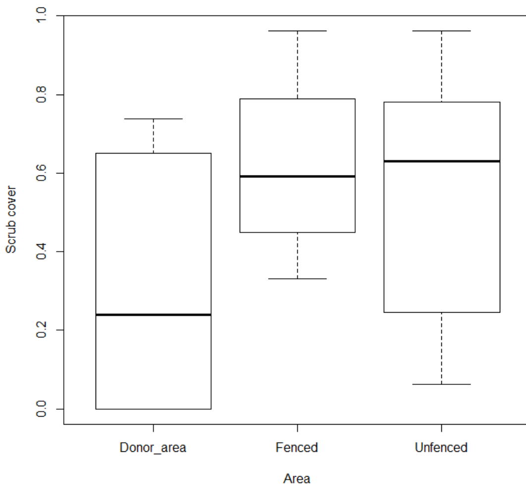
Figure S1. Boxplots of scrub cover for the different areas. ANOVA of comparison among study areas: F_{2,17} = 2.185 , P = 0.143 .
