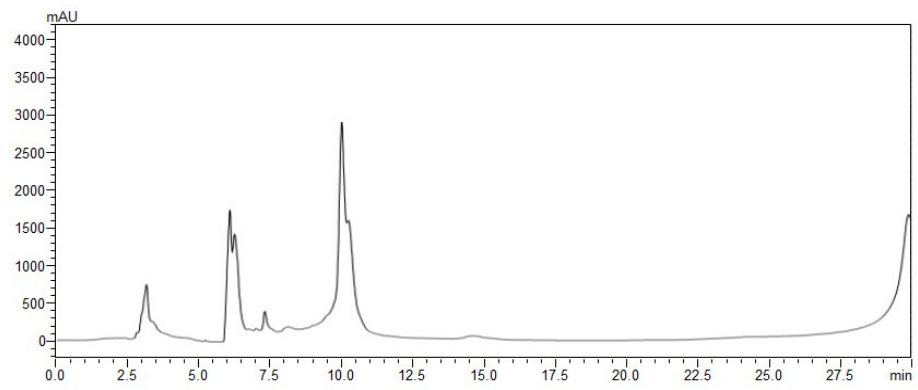
(e) Chromatogram of Cu-3 treated plants
