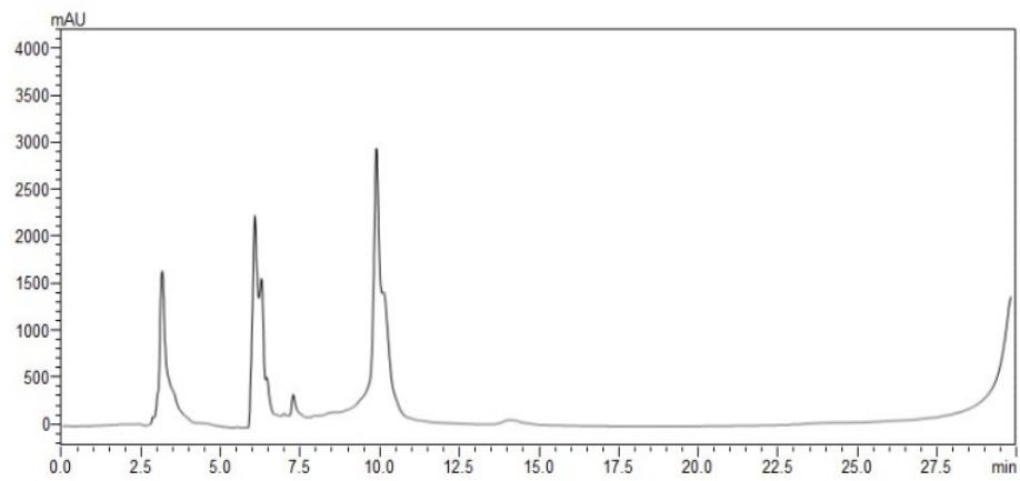
(f) Chromatogram of Cu-4 treated plants
