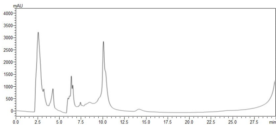
(i) Chromatogram of Fe-3 treated plants
