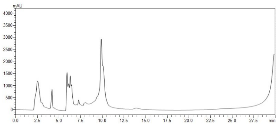
(h) Chromatogram of Fe-2 treated plants
